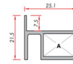
Single Glass Panel Tek Cam Paneli
