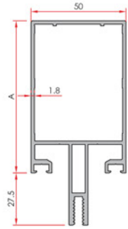
1.8 mm Mullion Profiles 1.8 mm Mulyon Profilleri
