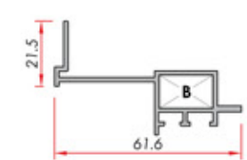
Composite Panel Kompoze Paneli
