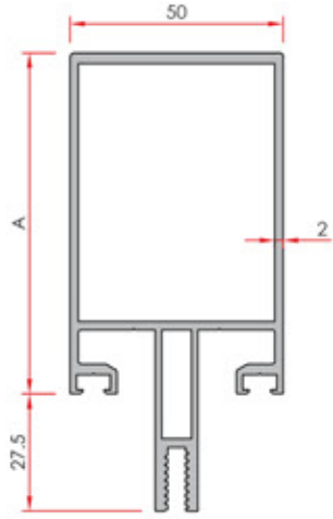
2 mm Mullion Profiles 2 mm Mulyon Profilleri
