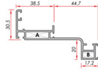
Hidden Wing Frame Gizli Kanat Kasa Paneli
