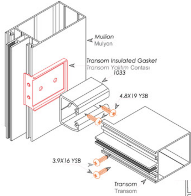
Glass Facade System Which Cover Combination Kapaklı Cephe Sistemi Fitil Cam Kombinasyonu
