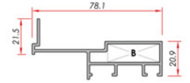
Composite Panel Kompoze Paneli
