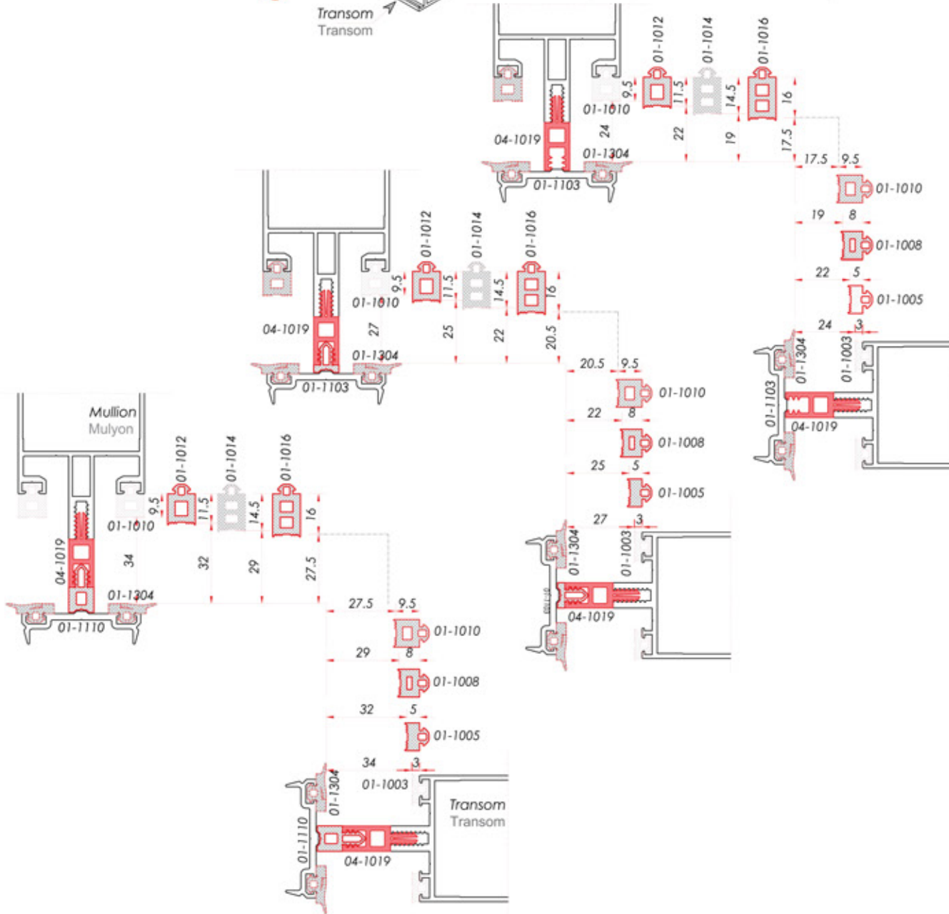
Glass Facade System Which Cover Combination Kapaklı Cephe Sistemi Fitil Cam Kombinasyonu
