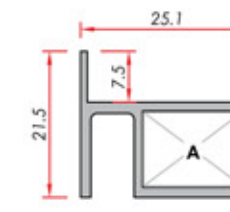
Single Glass Panel Tek Cam Paneli
