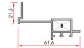
Composite Panel Kompoze Paneli
