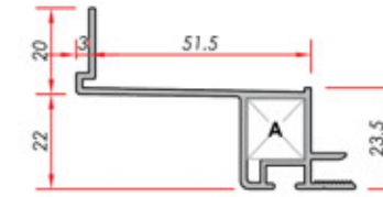
Composite Panel Kompoze Paneli
