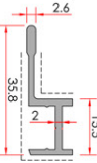
Swapper Rail Profile Sineklik Profili
