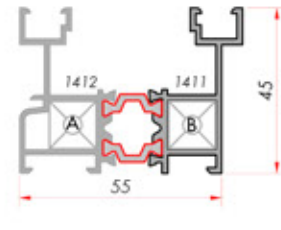
Two Rail Frame İki Raylı Kasa
