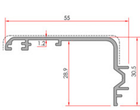
Window Sill Pervaz Profili
