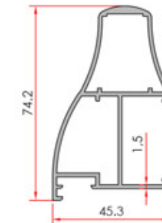
Reinforced Vent Takviyeli Kanat
